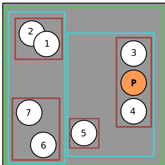
Figure 181: Example of a search in an AABB-Tree
